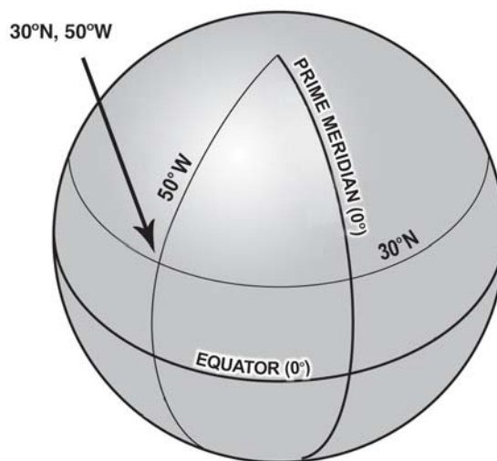
Figure 3-2. The coordinates for the point where latitude and longitude meet are described as 30^\circ N, 50^\circ W.
